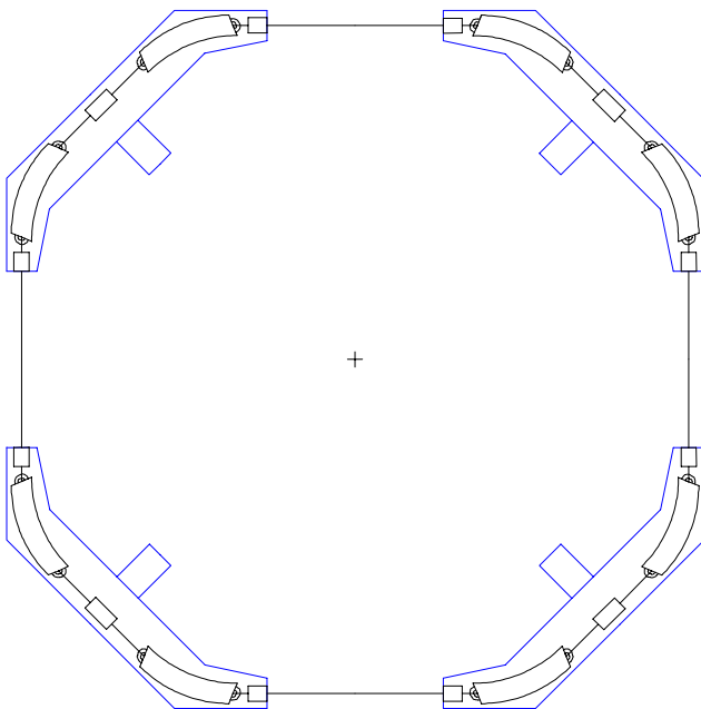
Figure 2. Layout of the two rings.
